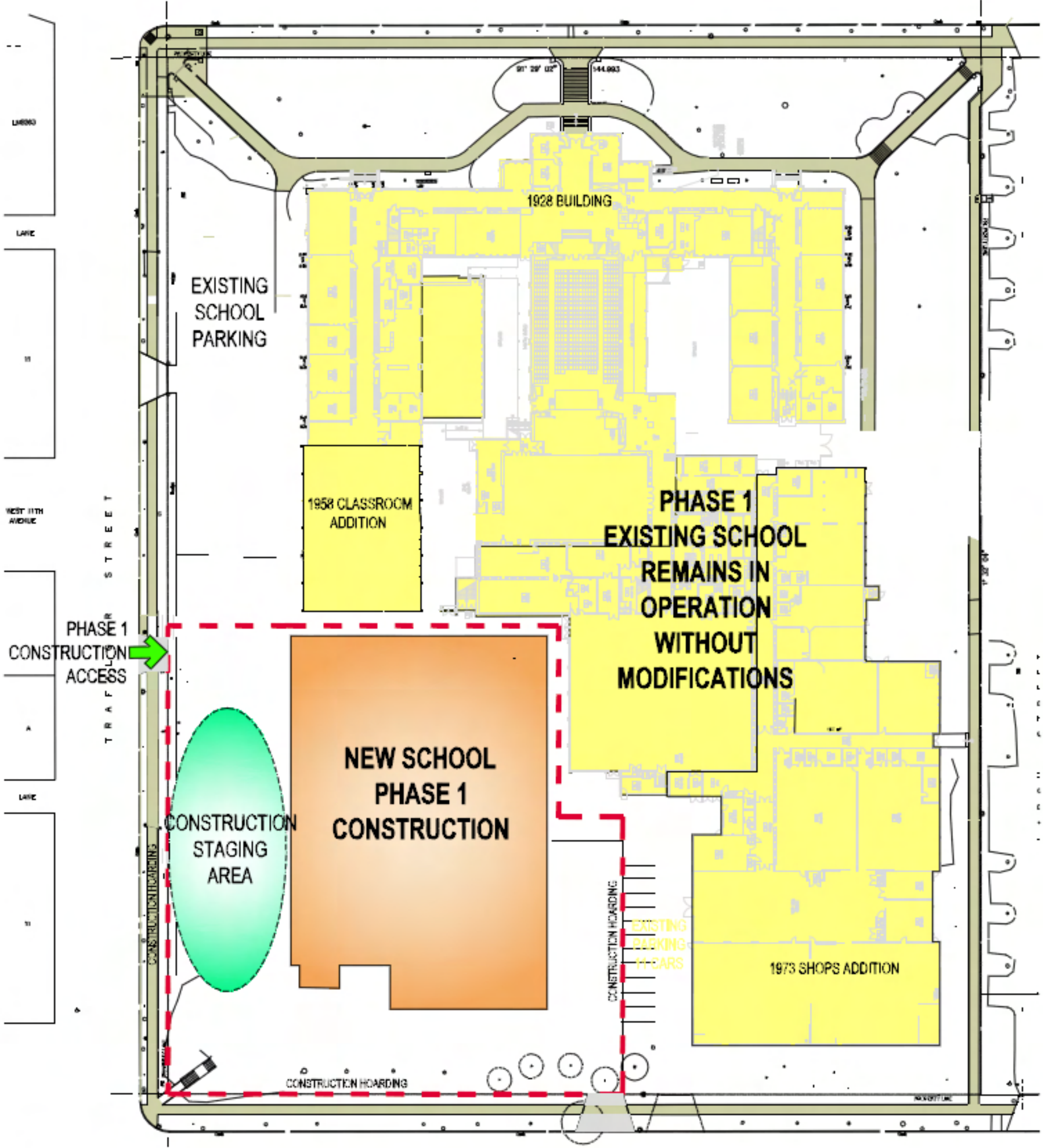
CONSTRUCTION PHASE 1 MASTER BUILDING PERMIT STAGE 1 - CONSTRUCTION OF SOUTH WING OF NEW 3 STOREY BUILDING
